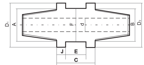
Pin-Pin Adapters
