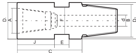
Pin-Box Adapters
